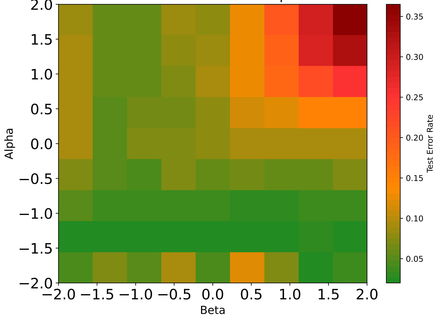
Test Error Rate for Different Alpha-Beta
